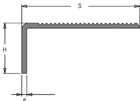
NDM VDi strié / NDM VDi striped
